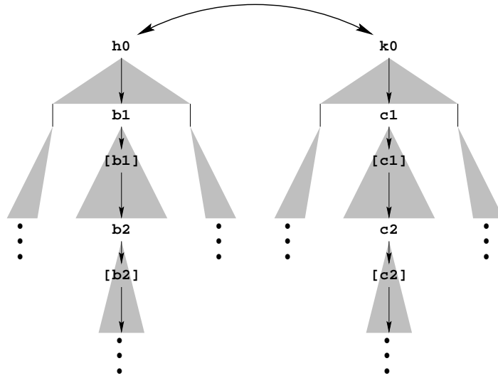
Figure 3: The clock hierarchy computed by the DC + or SIGNAL compiler.
