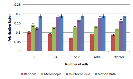
Figure 9: Polarization scores of different sampling techniques on various discretizing scales comparing to the motion data.
