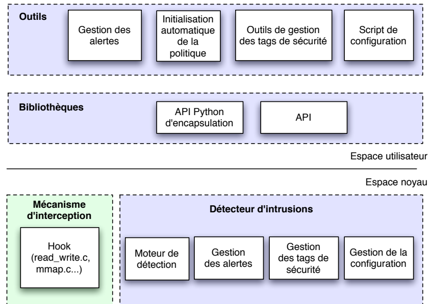
FIG. 3.5 – Architecture de Blare
