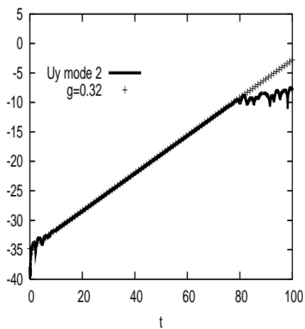
Figure 9: Time evolution of the second mode of U_y .
