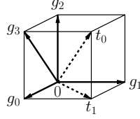
Fig. 1. The sets \mathcal{G} and \mathcal{T} from Example 5.
