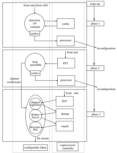
Fig. 3. 802.11 baseband receiver with the 3 main phases triggered by microcontroller (short and long preamble detection, then payload)
