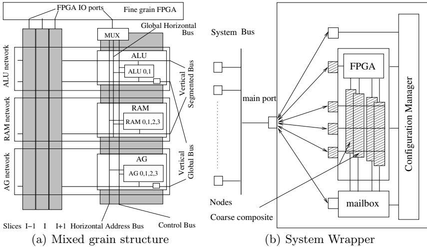
Fig. 2. Two architecture views
