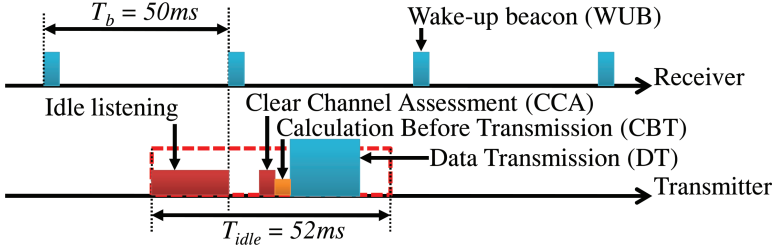
Fig. 8. Communication protocol between two nodes. When waking up, the transmitter waits for a wake-up beacon (WUB) from the receiver. After receiving a WUB, the transmitter forwards data packet (DT) after clear channel assessment (CCA) and calculation before transmission (CBT).
