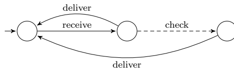
Fig. 1 Modal transition system modeling a simple email system, with an optional behavior: Once an email is received it may e.g. be scanned for containing viruses, or automatically decrypted, before it is delivered to the receiver.
