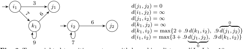
Fig. 6 Two weighted transition systems with branching distance d(I_1, I_2) = 18 .
