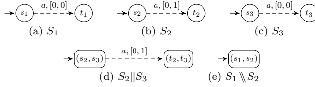
Fig. 11 WMTS for which d_m(S_2||S_3, S_1) \neq d_m(S_3, S_1 \parallel S_2) = \infty .
