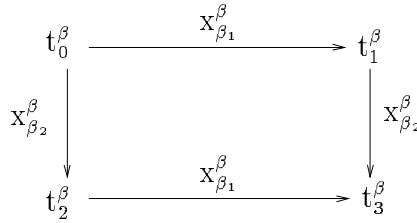
Figure 2: T^\beta
