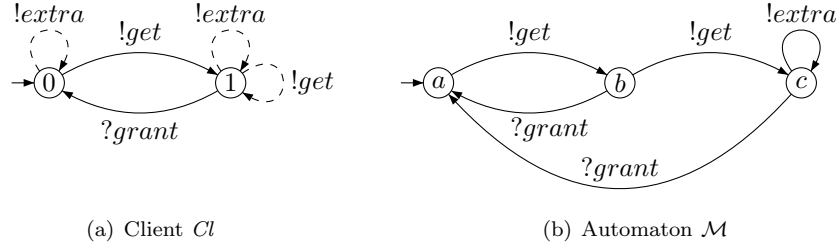
Figure 1: The modal specification Cl accepts the automaton \mathcal{M}
